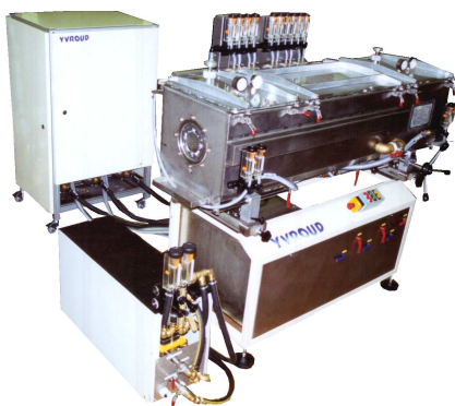
2 Chambers calibrating tank model BCV20 with closed circuit and movable spraying box For cosmetic pipes Ø max 60
