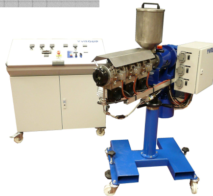
Various coextruders diam 18 to 30 mm With separated or stand on electrical cabinet
