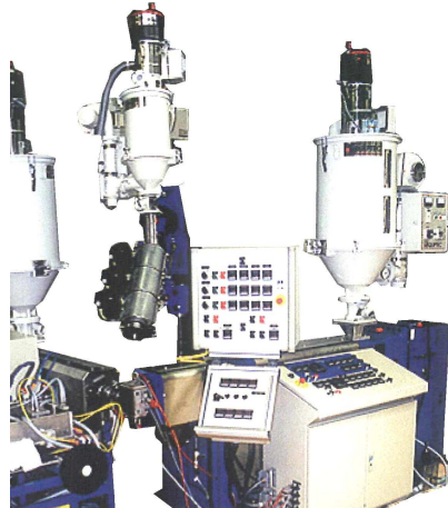
Co-extrusion head For multilayer pipe
